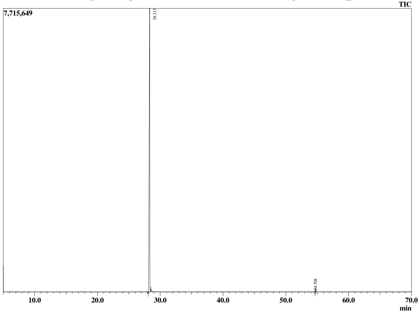
Chromatogram Wintergreen C:\GCMSsolution\Data\EOU\Academic\Wintergreen B151008K.qgd
